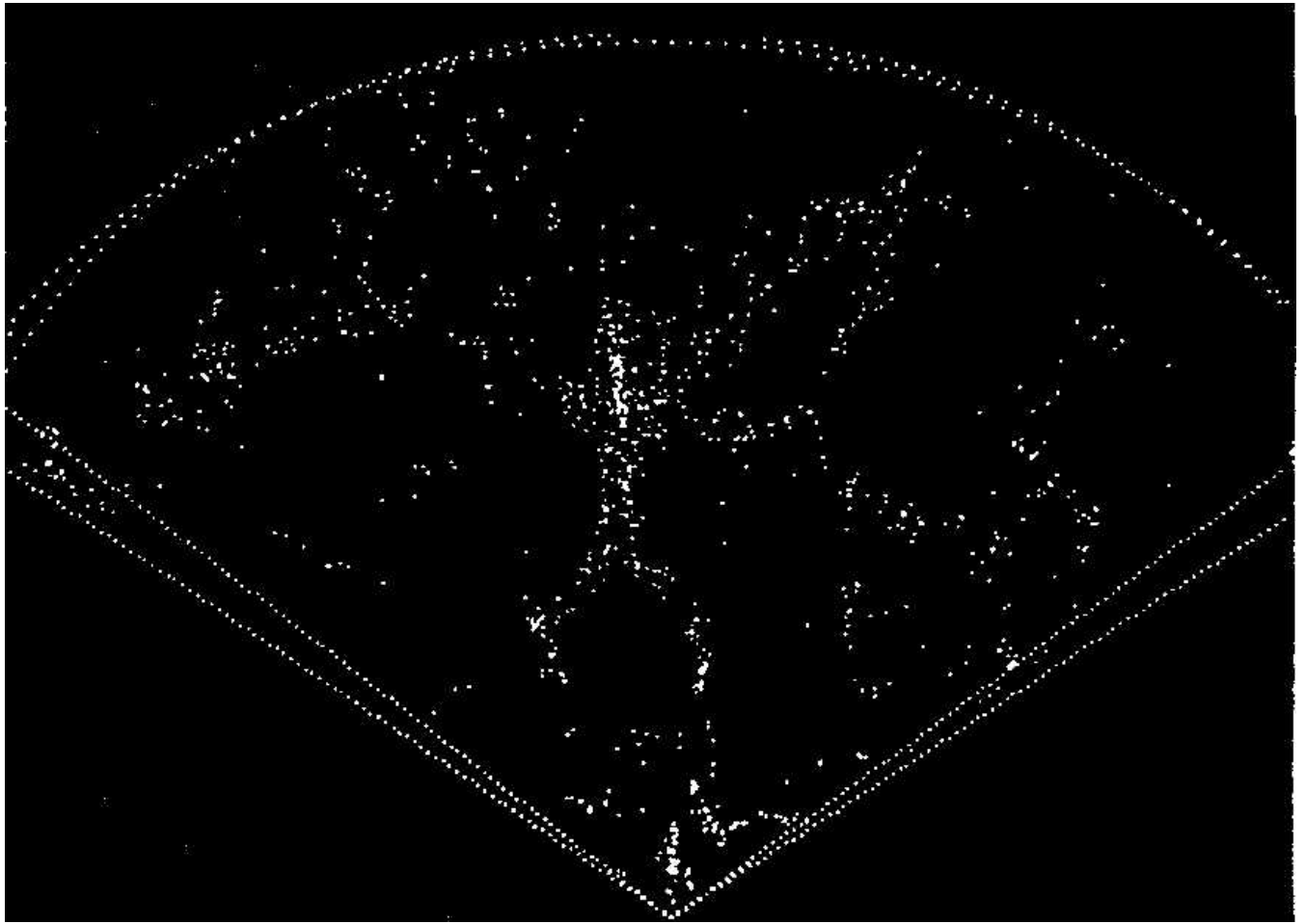
Fig. 11. A three-dimensional map showing a wedge of the Universe . This map was prepared at the Centre for Astrophysics, Harvard College Observatory and Smithsonian Astrophysical Observatory, by Margaret J. Geller, John P. Huchra and Valérie de Lapparent. It was published in Scientific American , March 1986 (Vol. 254, Number 3), page 49. The map reveals a cluster of galaxies which takes the apparent shape of a human figure. This human shape may gain special significance with the Concept of Dipolar Gravity stating that our universe is composed of two parallel worlds of a physical nature (i.e. the world of matter and the counter-world), which exactly copy each other like an object and its mirror reflection. The non-material one of these two worlds (i.e. the counter-world) is made of a substance (counter-matter) that is able to think in its natural constitution. This thinking substance forms the universal computer (UC) described in subsection I3.2, whose shape and dimensions must reflect the shape of our universe, and whose capabilities correspond to those of God. This in turn invokes a question as to whether the above human shape is a pure coincidence or astronomic confirmation to the biblical statement that "God created man in his own image".
